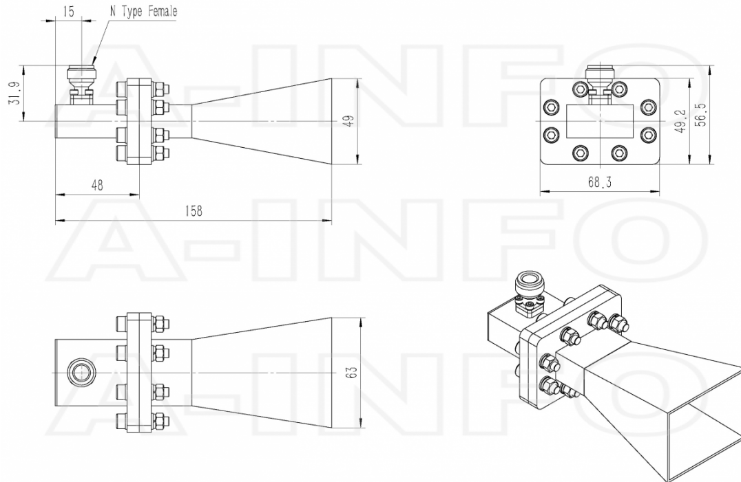
N-Female Output (P/N: LB-137-10-C-NF)
